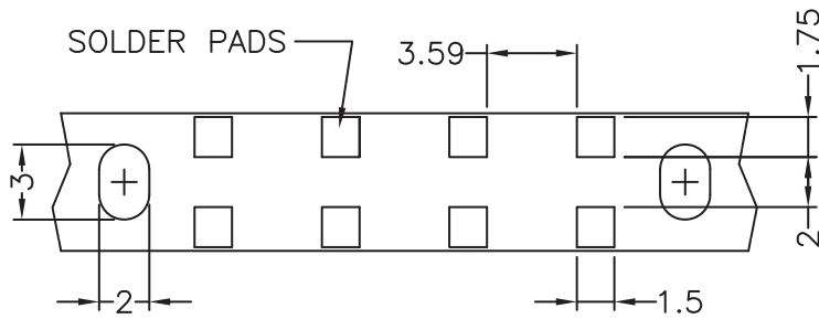
PCB LAYOUT
