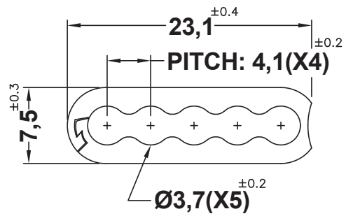
UNIT FOLDED VIEW
